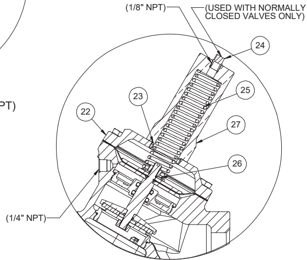
1072485 (VAVF-0002-90000) (2\" NPT) SPRING ASSIST CLOSED
