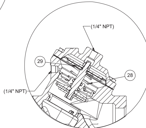
1072484 (VAVF-0001-90000) (2\" NPT) SPRING ASSIST OPEN
